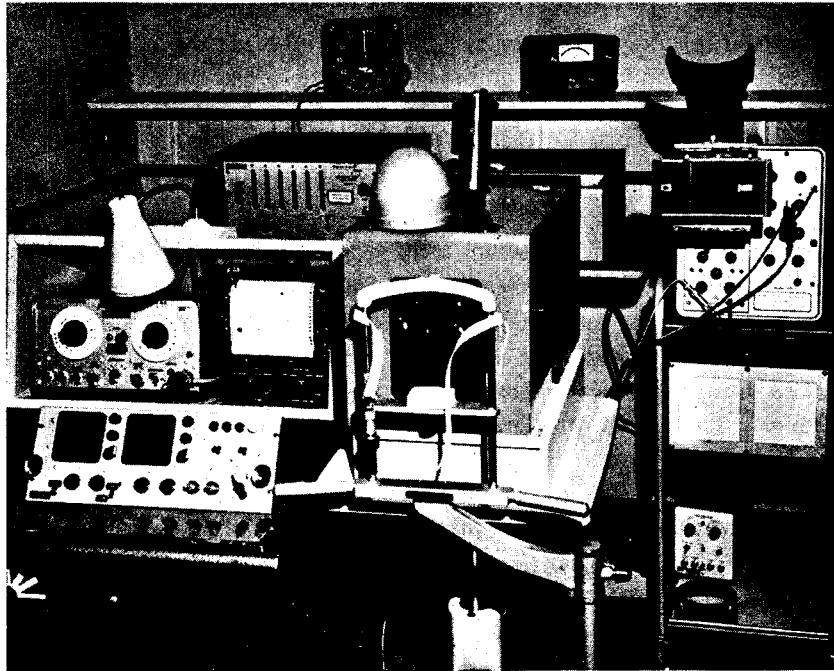
Figure 3. Photo of test apparatus.
